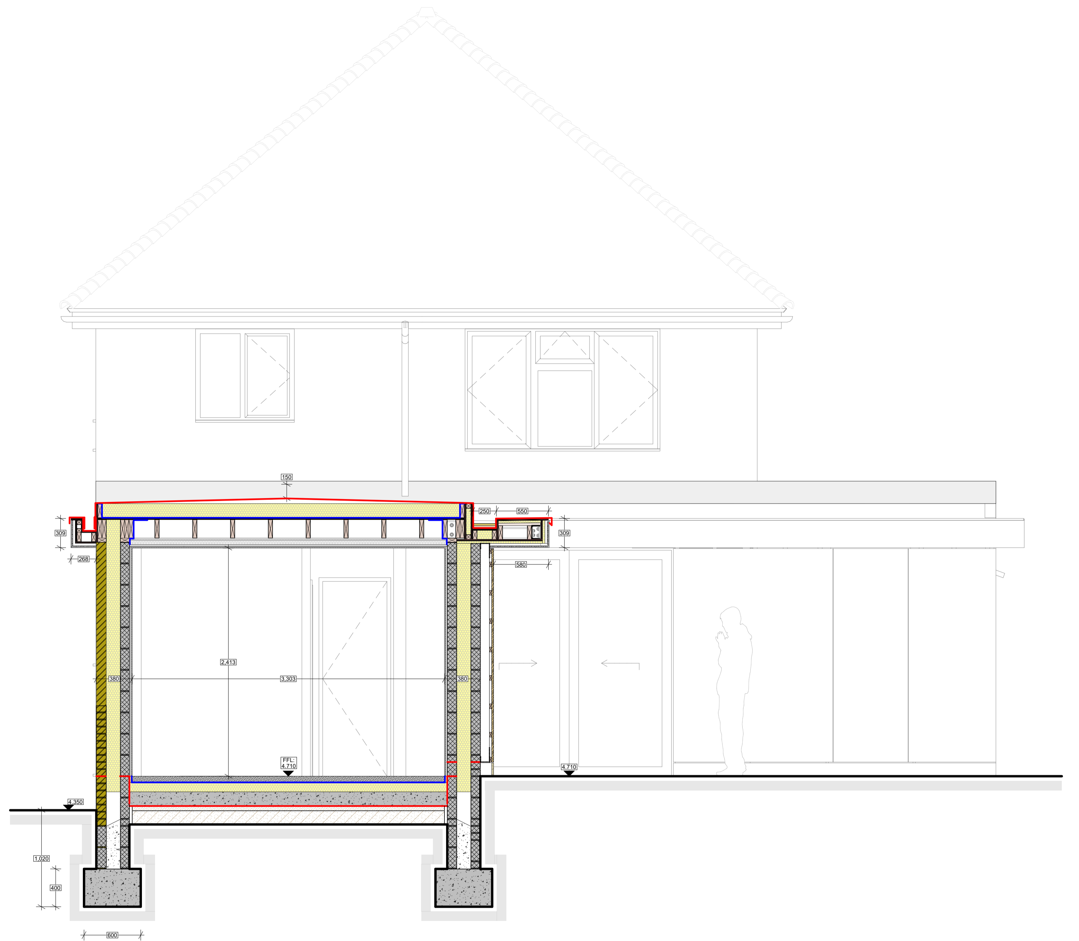
S02 Technical Cross Section + Outline Elevation 1:25
