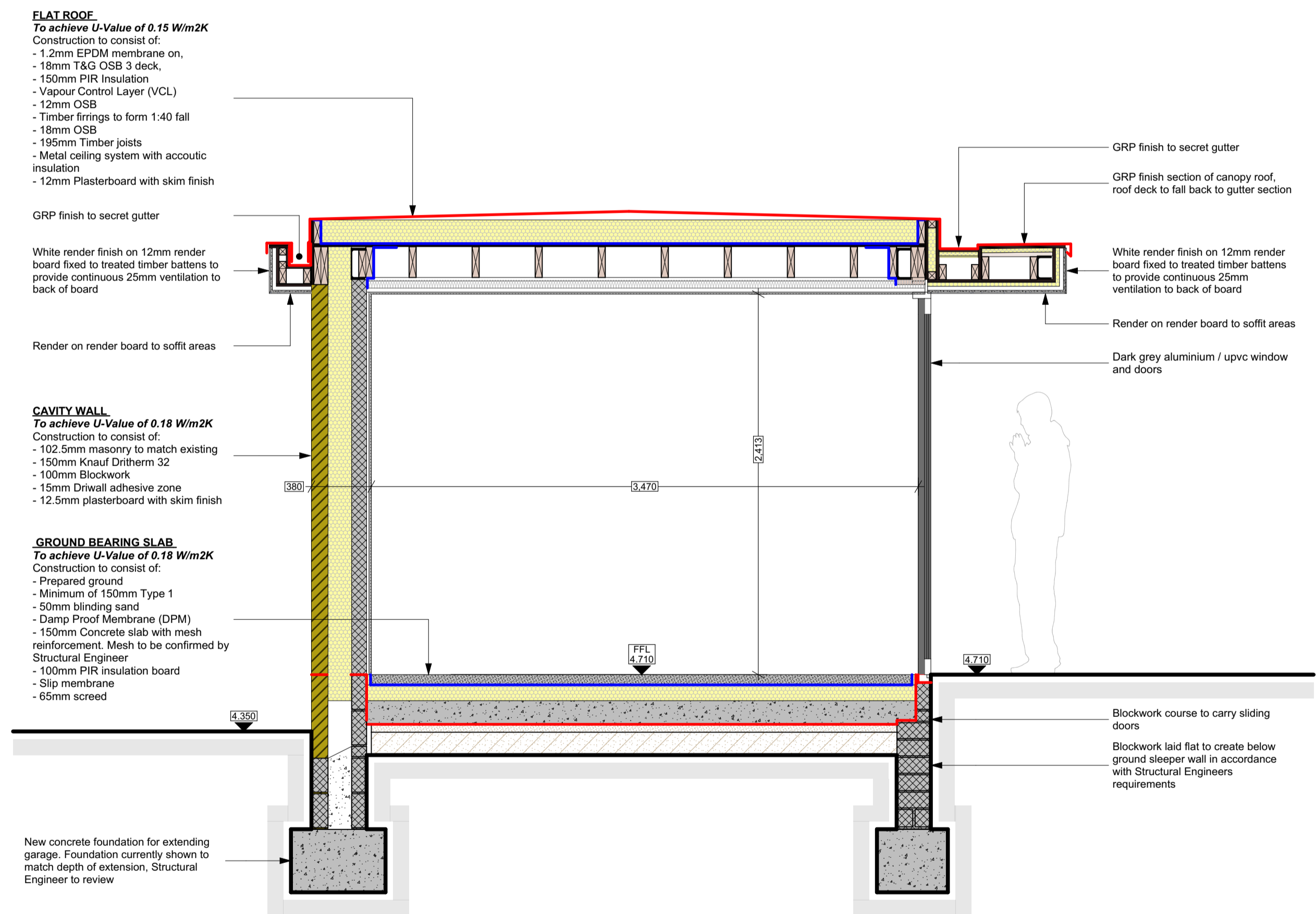
S01 Technical Cross Section 1:25
